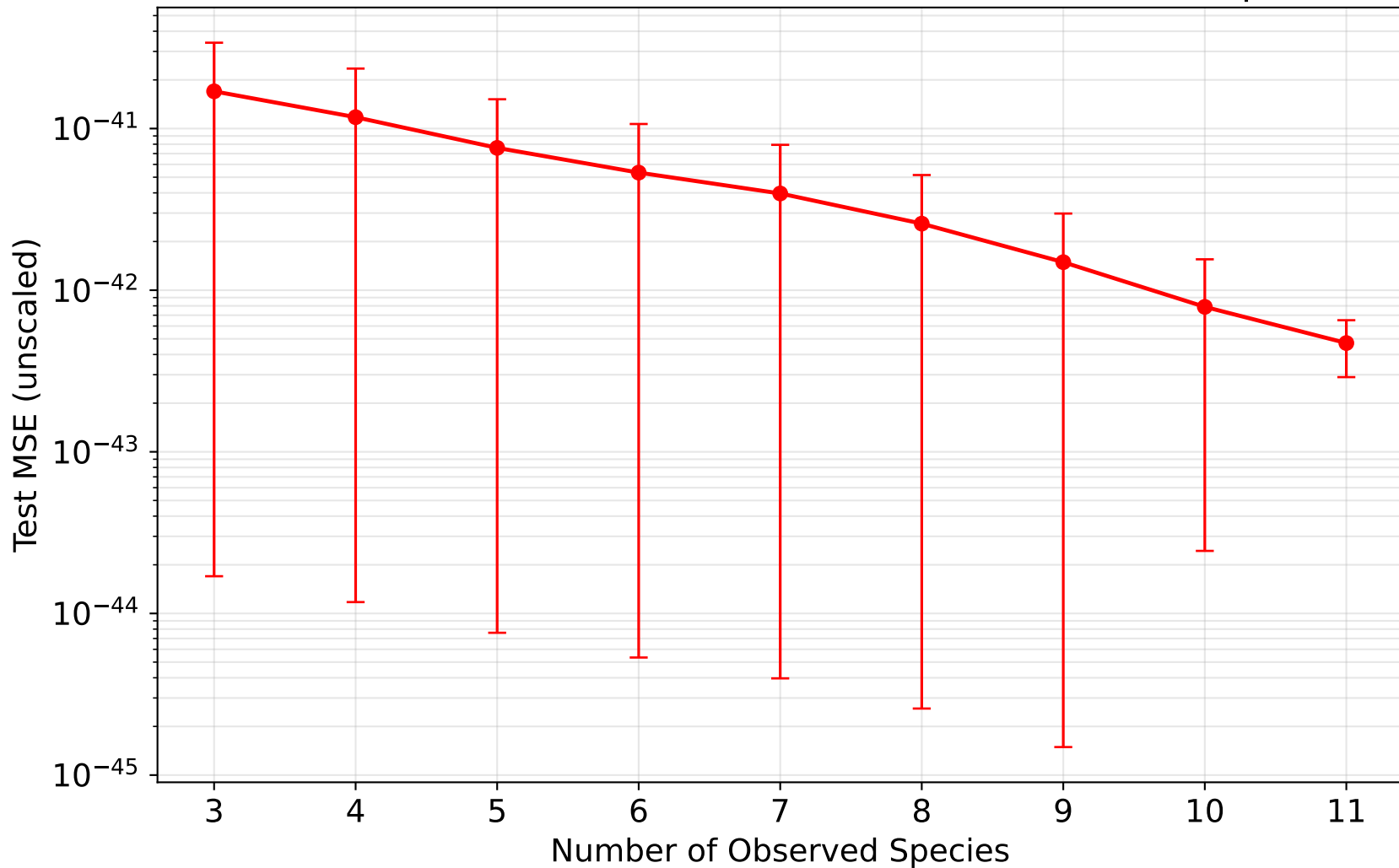
50, 50 — Test MSE (unscaled) vs number of observed species
